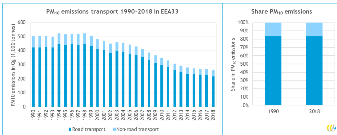
Figure 11 - Trends in PM 10 emissions from 1990-2018 (EEA, 2020a)
