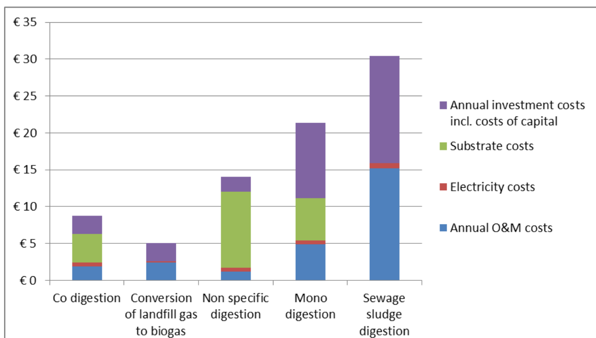
Figure 20 Scenario 3: break down of EU28 average production costs in 2030 of biogas (incl. investments) over period 2015-2030 in €/GJ
